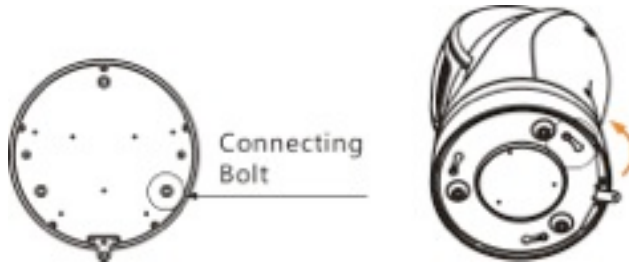
Fig. 8: Mount the Installation Plate
