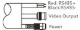
Fig. 13: Cable Connection 2
