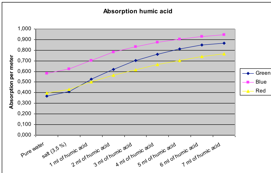
Figure 4. Graph showing light absorption per meter for increasing concentrations of humic acid.
