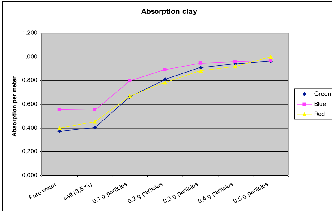
Figure 3. Graph showing light absorption per meter for increasing concentration of clay.
