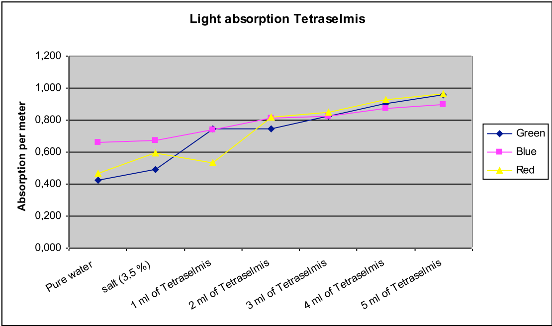
Figure 1. Graph showing light absorption per meter for increasing concentration of the algae Tetraselmis.
