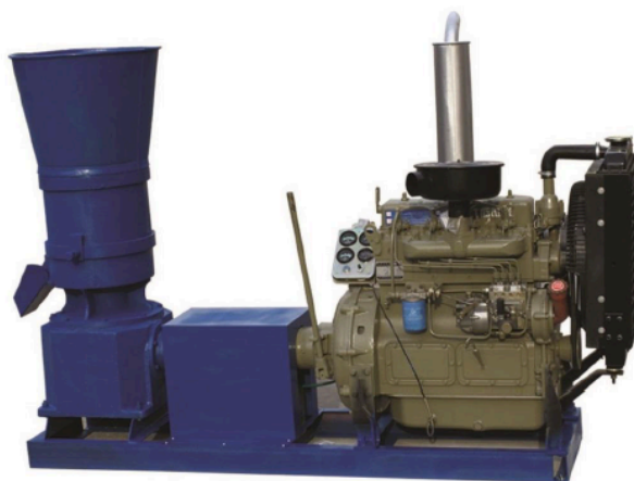
Pellet Mill
